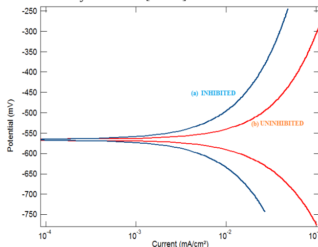
Fig -3: Potentiostatic polarization diagram of steel in (a) mixed type inhibited (b) uninhibited solution
